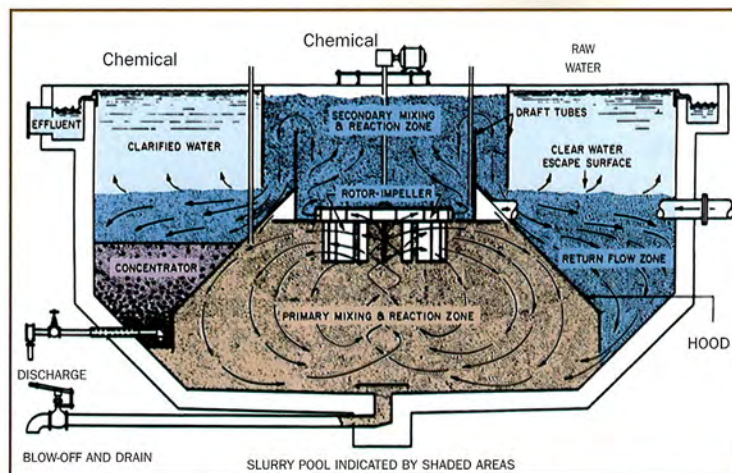
Solids-contact clarifier
