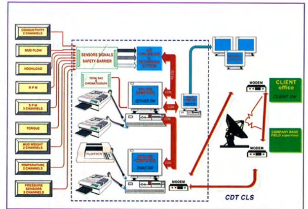
CDT Compact Logging System ( CLS )
